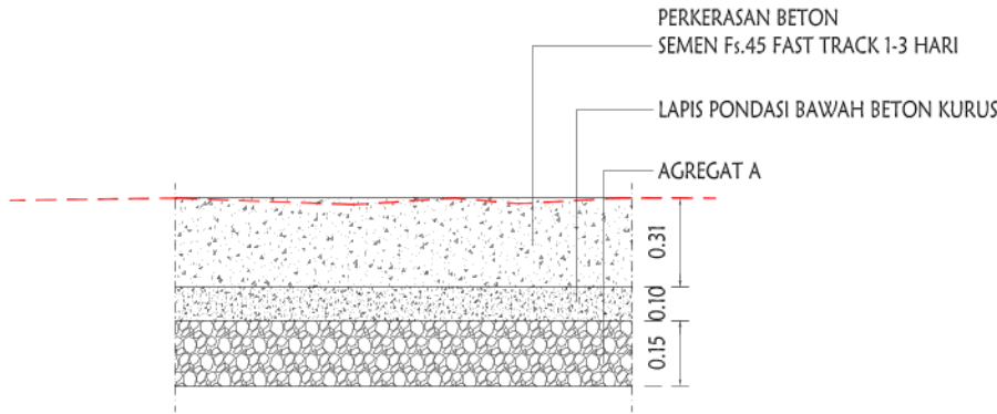
DETAIL PERKERASAN SKALA 1: 25
