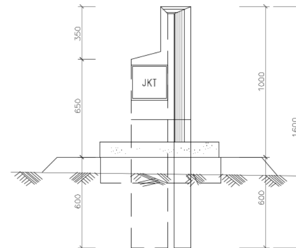
TAMPAK SAMPING
