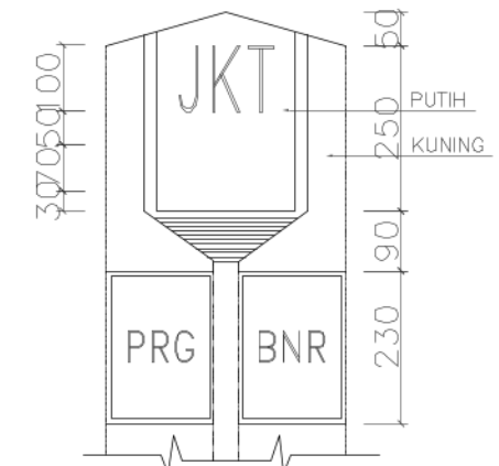
DETAIL 1
