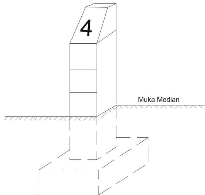
ISOMETRIS
