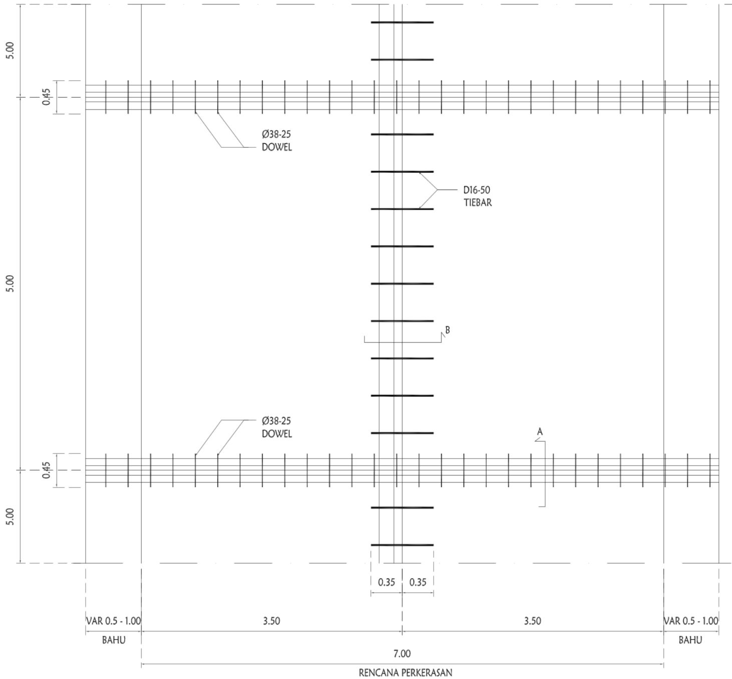
DENAH PERKERASAN BETON SKALA 1: 50
