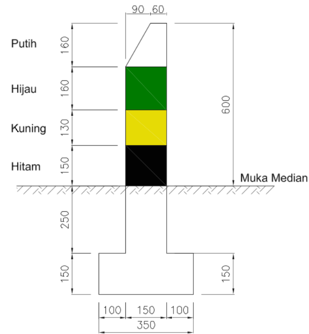
TAMPAK SAMPIING
