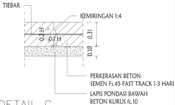
DETAIL C SKALA 1: 25
